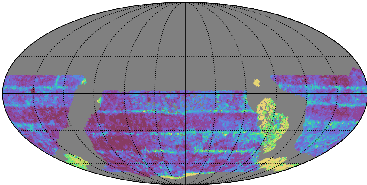
too_100_4v3.4_10yrs WFD z band: Median Inter-Night Gap
