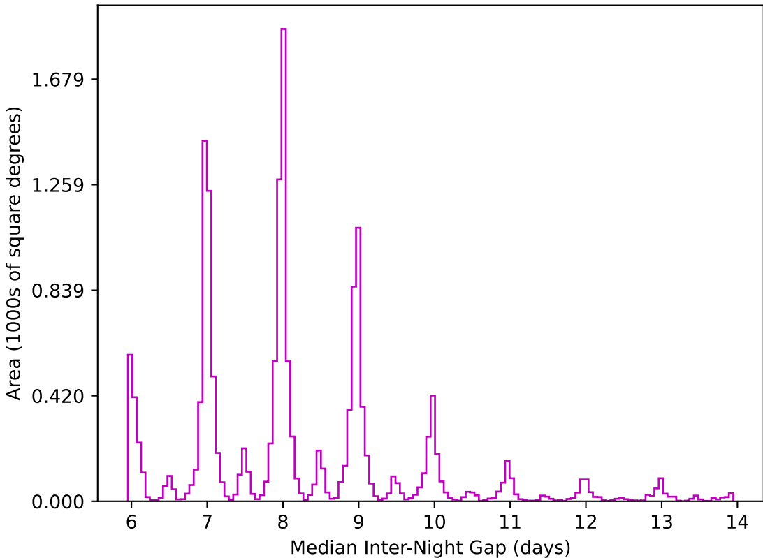
too_100_4v3.4_10yrs WFD z band: Median Inter-Night Gap
