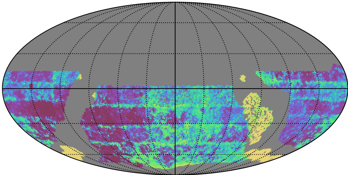
too_100_4v3.4_10yrs WFD y band: Median Inter-Night Gap
