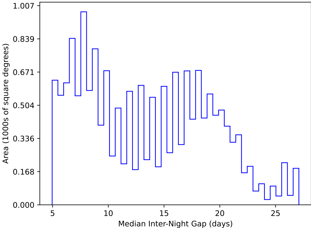
too_100_4v3.4_10yrs WFD y band: Median Inter-Night Gap
