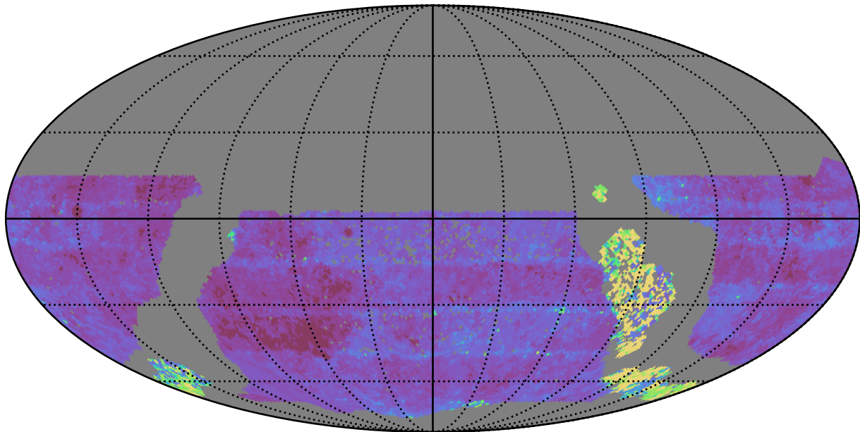
too_100_4v3.4_10yrs WFD u band: Median Inter-Night Gap
