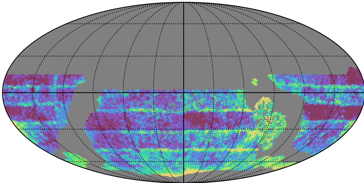
too_100_4v3.4_10yrs WFD r band: Median Inter-Night Gap
