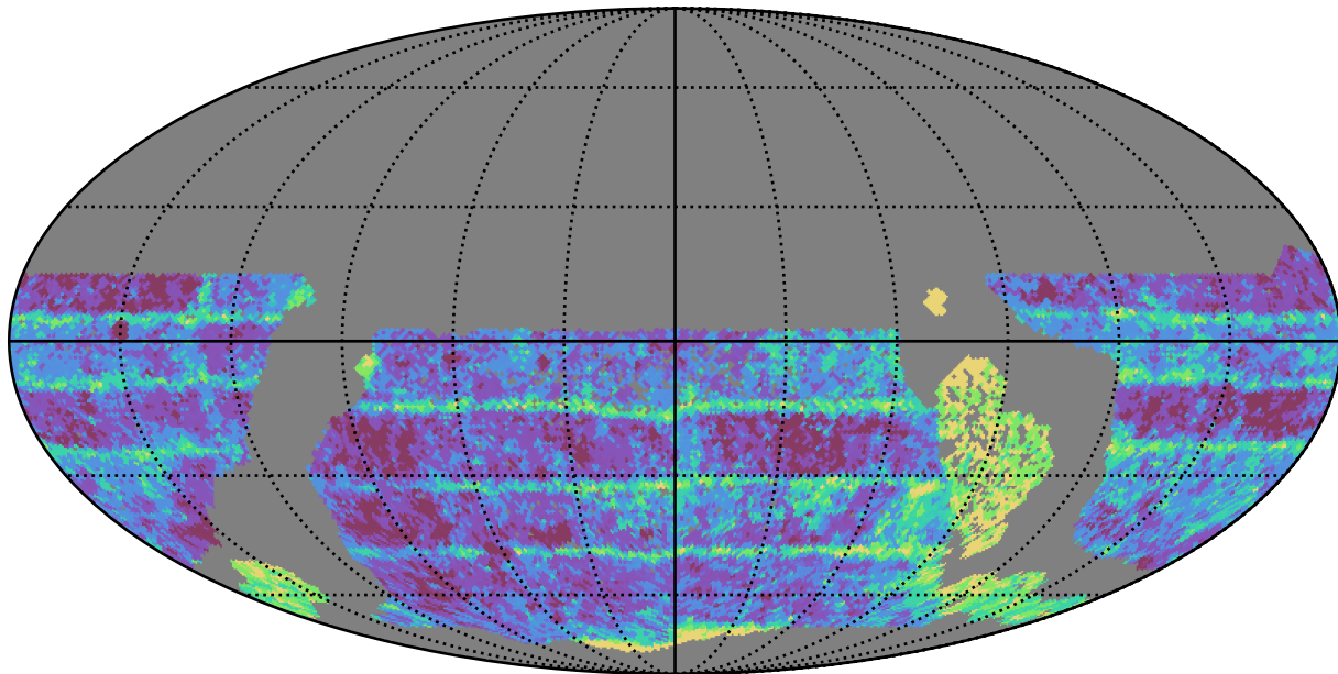
too_100_4v3.4_10yrs WFD i band: Median Inter-Night Gap
