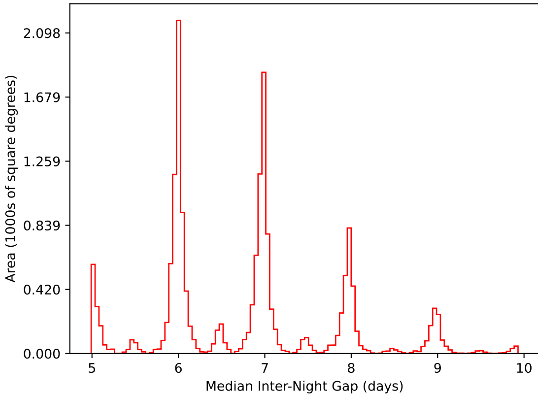
too_100_4v3.4_10yrs WFD i band: Median Inter-Night Gap
