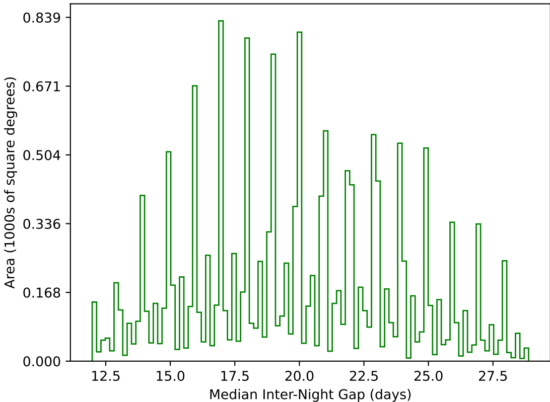
too_100_4v3.4_10yrs WFD g band: Median Inter-Night Gap
