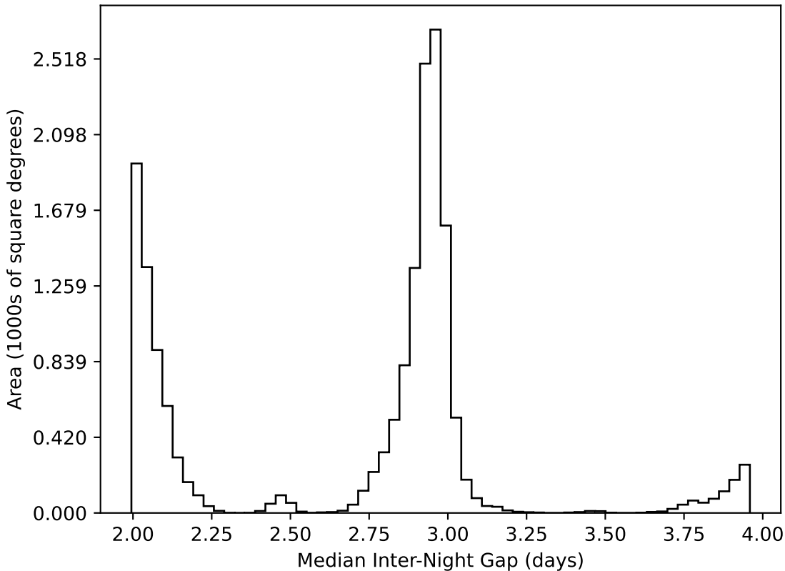
too_100_4v3.4_10yrs WFD all bands: Median Inter-Night Gap
