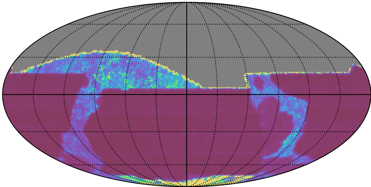
too_100_4v3.4_10yrs All sky z band: Median Inter-Night Gap
