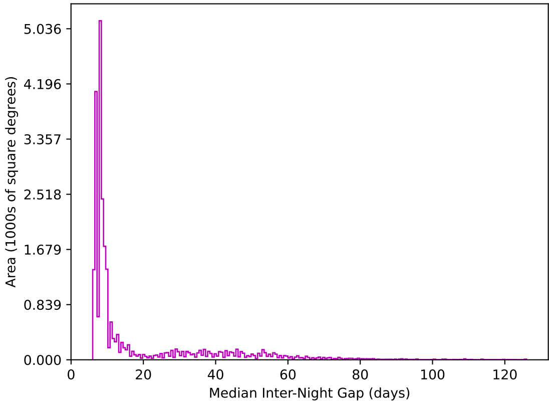
too_100_4v3.4_10yrs All sky z band: Median Inter-Night Gap
