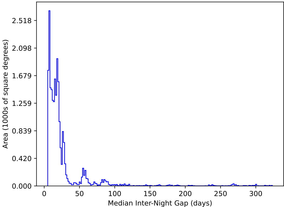
too_100_4v3.4_10yrs All sky y band: Median Inter-Night Gap
