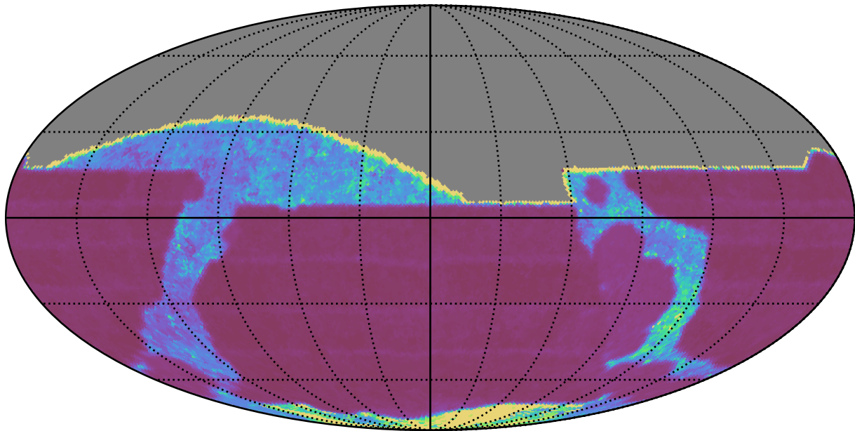
too_100_4v3.4_10yrs All sky i band: Median Inter-Night Gap
