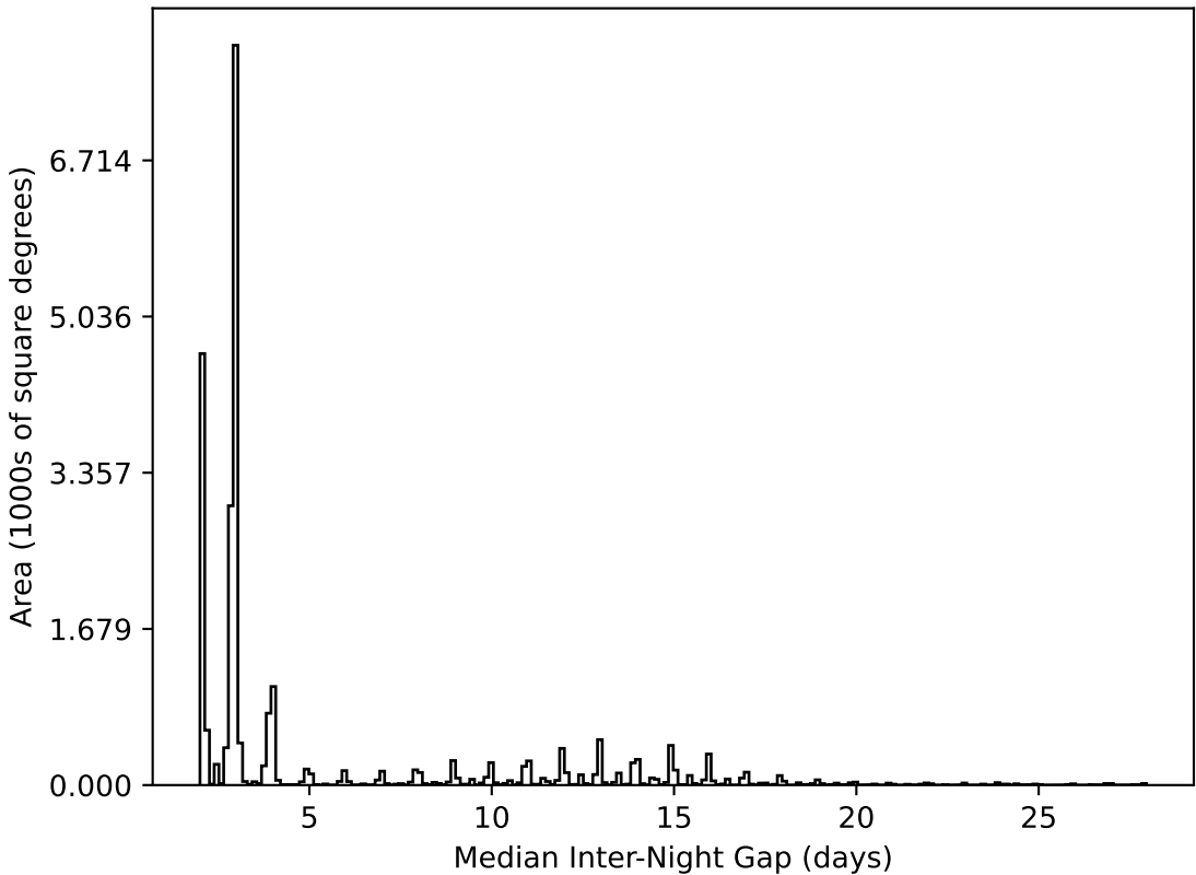
too_100_4v3.4_10yrs All sky all bands: Median Inter-Night Gap
