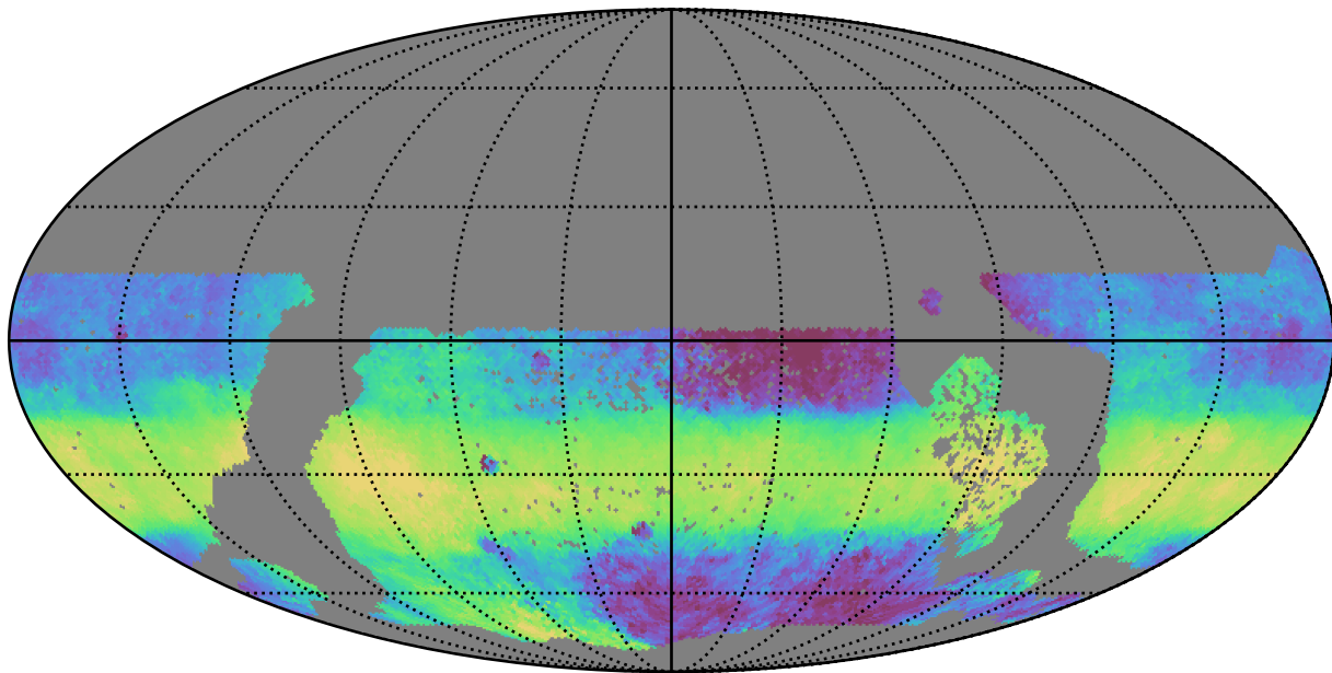
too_100_4v3.4_10yrs WFD y band: Median HA
