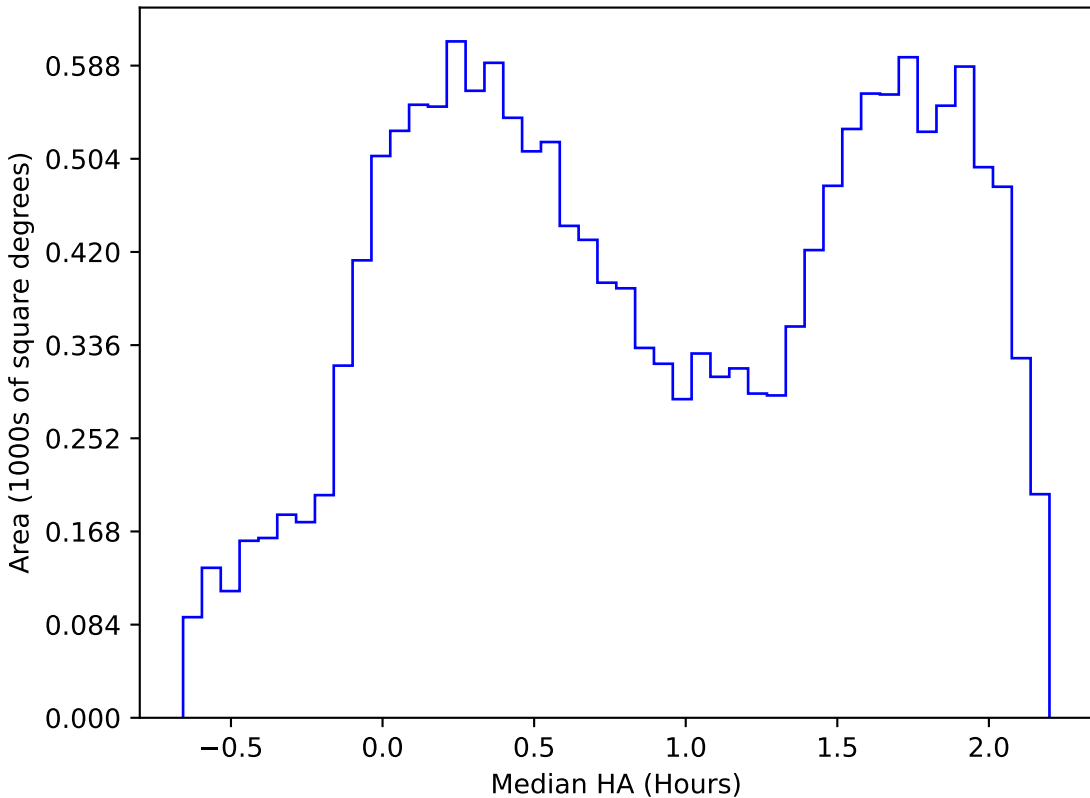
too_100_4v3.4_10yrs WFD r band: Median HA
