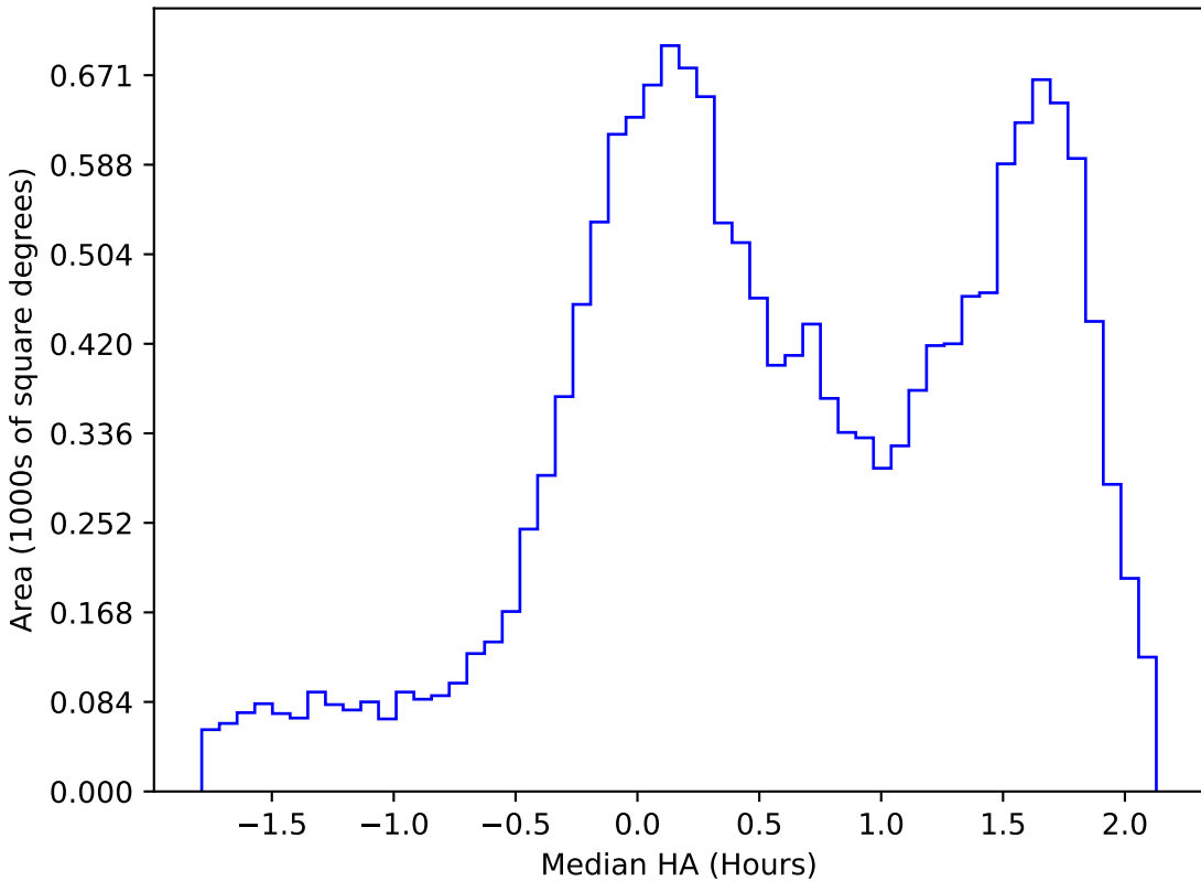
too_100_4v3.4_10yrs WFD g band: Median HA
