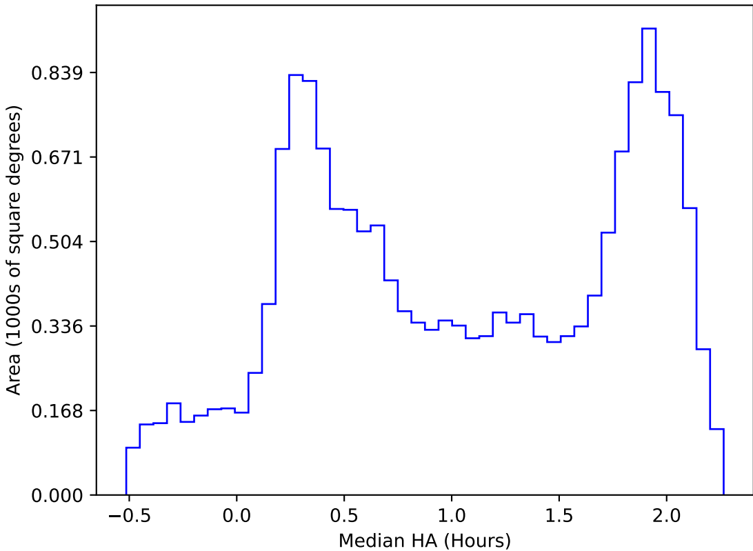
too_100_4v3.4_10yrs WFD all bands: Median HA
