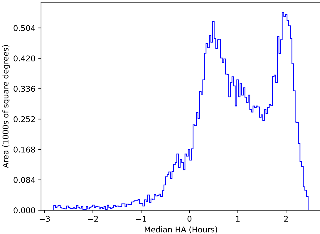
too_100_4v3.4_10yrs All sky z band: Median HA
