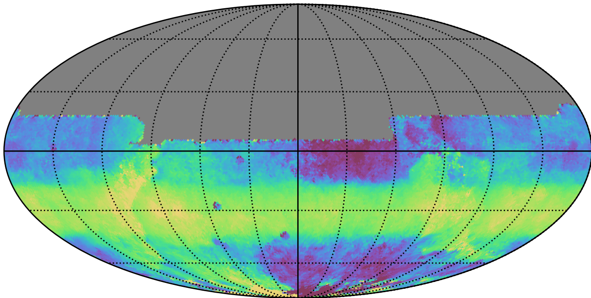
too_100_4v3.4_10yrs All sky y band: Median HA
