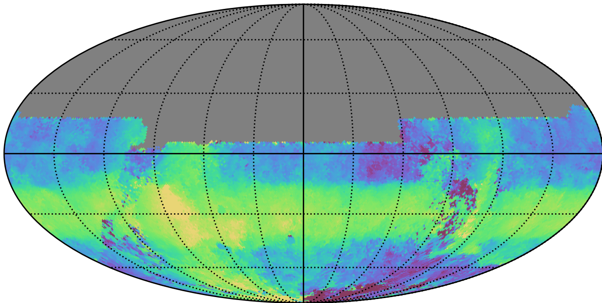
too_100_4v3.4_10yrs All sky u band: Median HA
