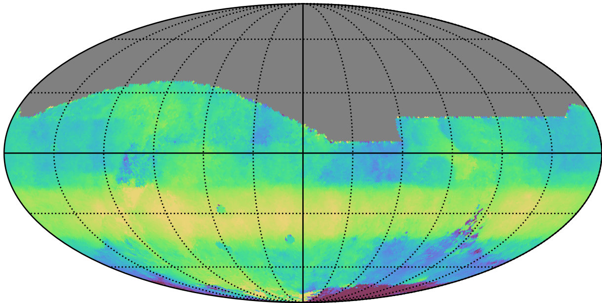
too_100_4v3.4_10yrs All sky r band: Median HA
