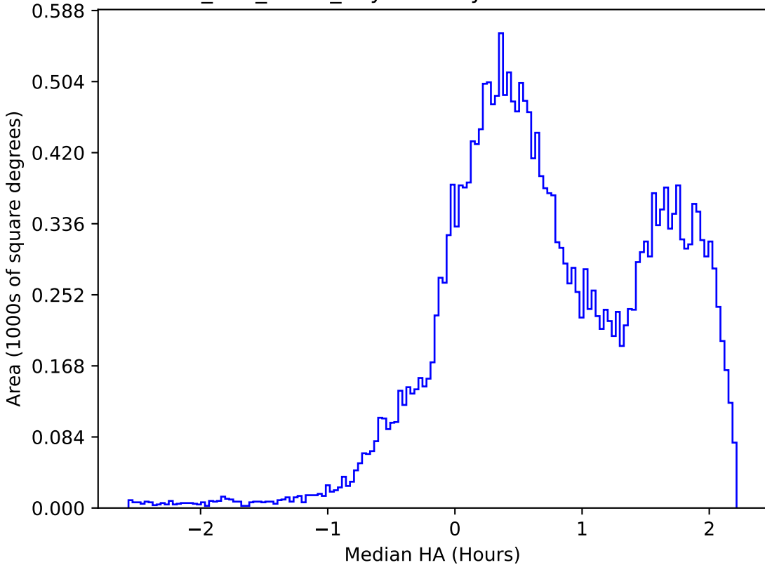
too_100_4v3.4_10yrs All sky r band: Median HA
