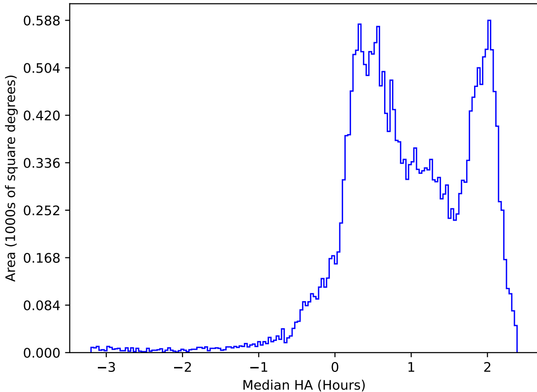
too_100_4v3.4_10yrs All sky i band: Median HA
