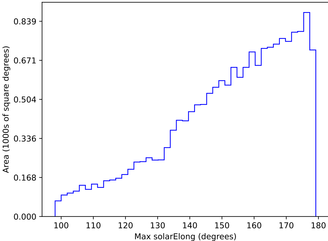
too_100_4v3.4_10yrs WFD u band: Max solarElong
