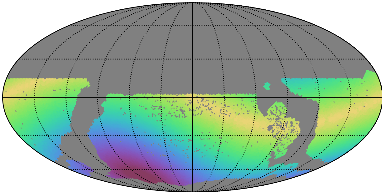
too_100_4v3.4_10yrs WFD g band: Max solarElong
