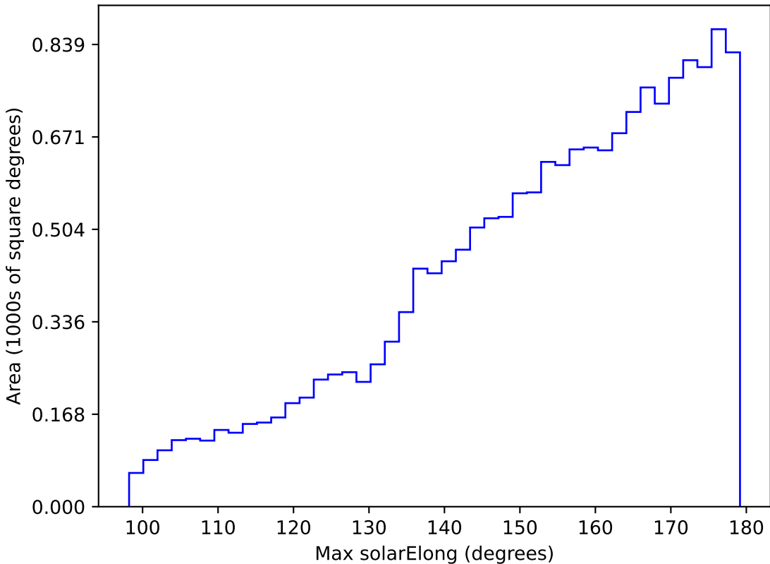
too_100_4v3.4_10yrs WFD g band: Max solarElong
