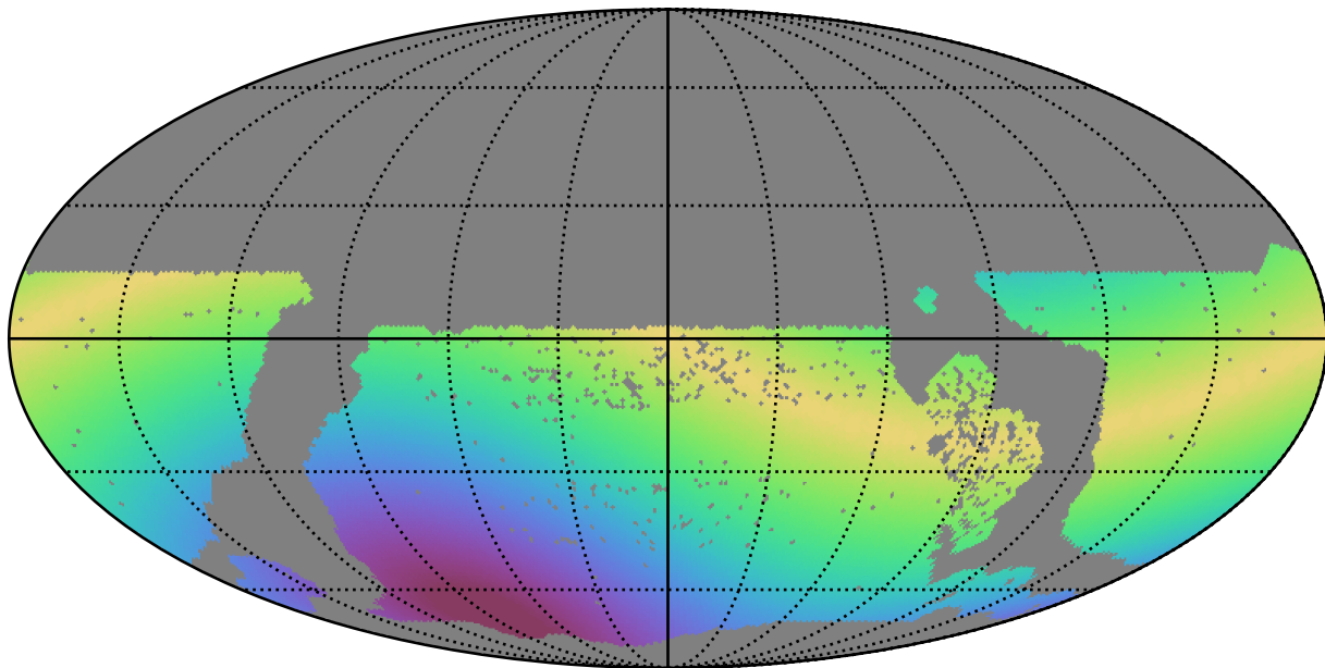
too_100_4v3.4_10yrs WFD all bands: Max solarElong
