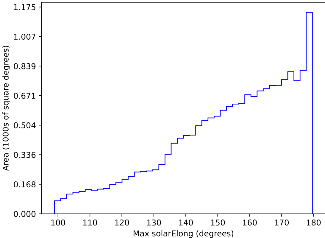
too_100_4v3.4_10yrs WFD all bands: Max solarElong
