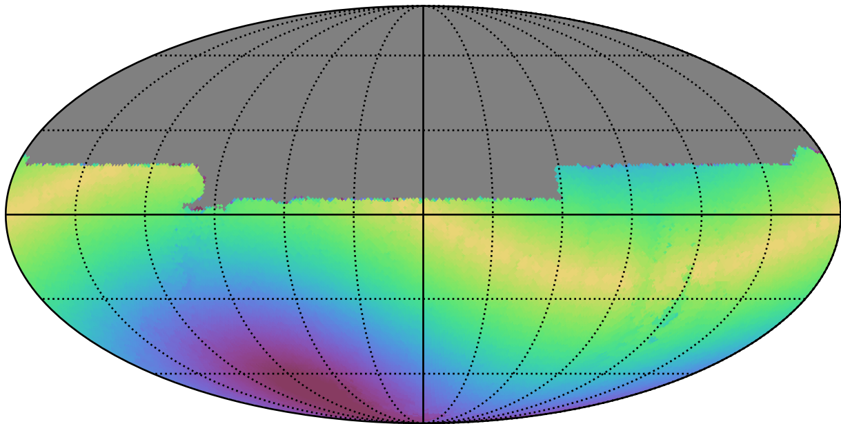
too_100_4v3.4_10yrs All sky u band: Max solarElong
