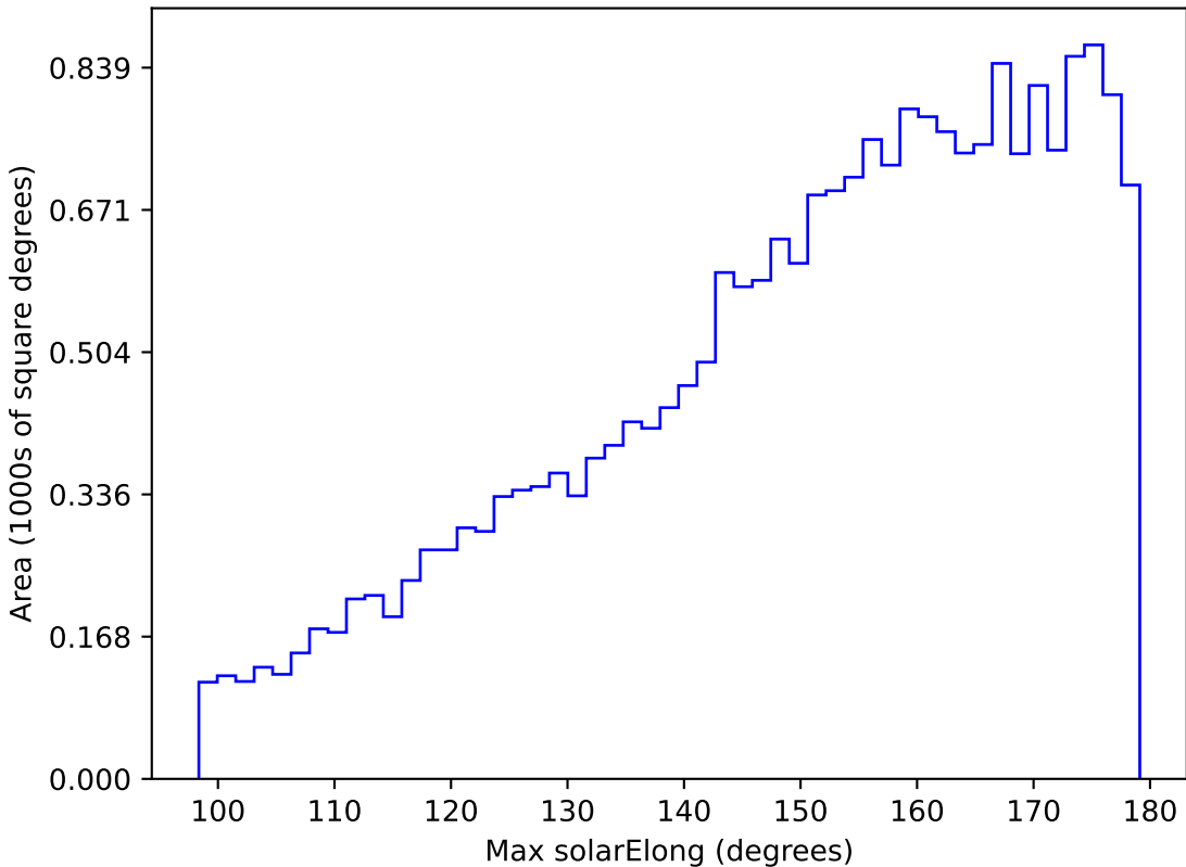
too_100_4v3.4_10yrs All sky u band: Max solarElong
