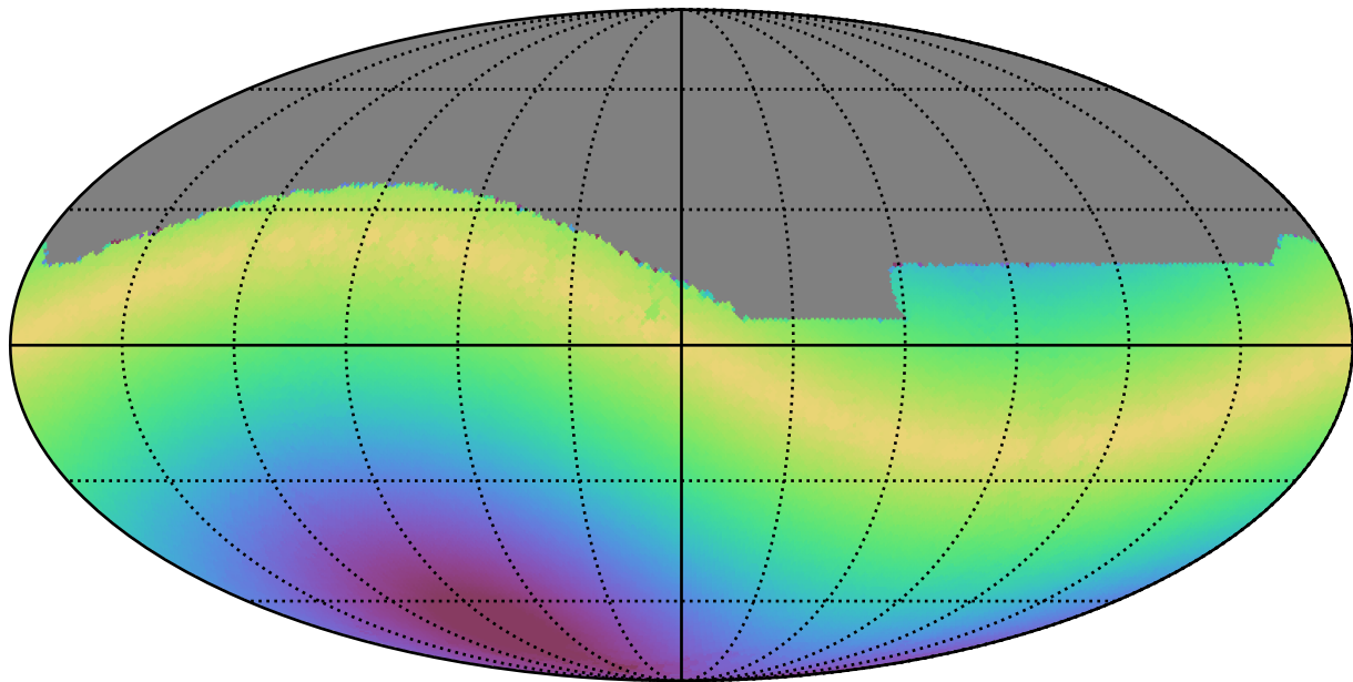
too_100_4v3.4_10yrs All sky r band: Max solarElong
