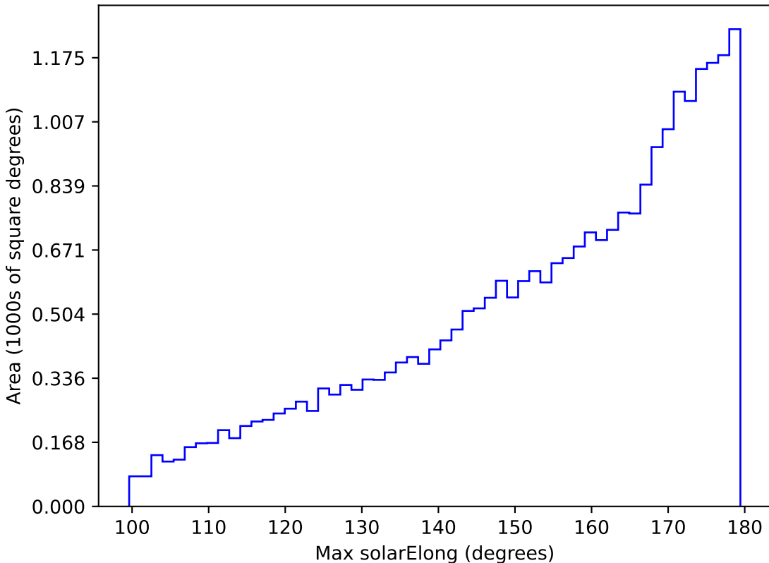
too_100_4v3.4_10yrs All sky r band: Max solarElong
