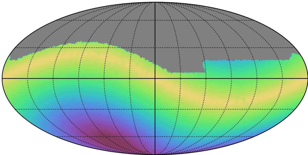
too_100_4v3.4_10yrs All sky i band: Max solarElong
