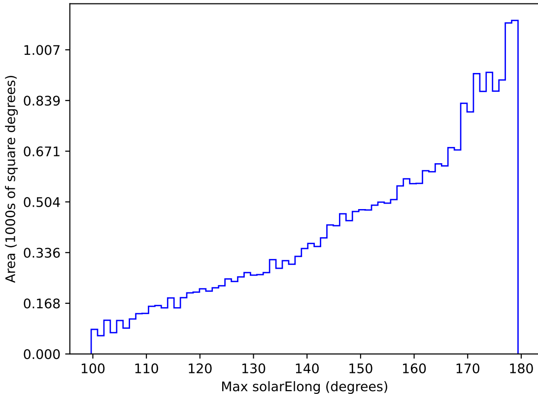
too_100_4v3.4_10yrs All sky i band: Max solarElong
