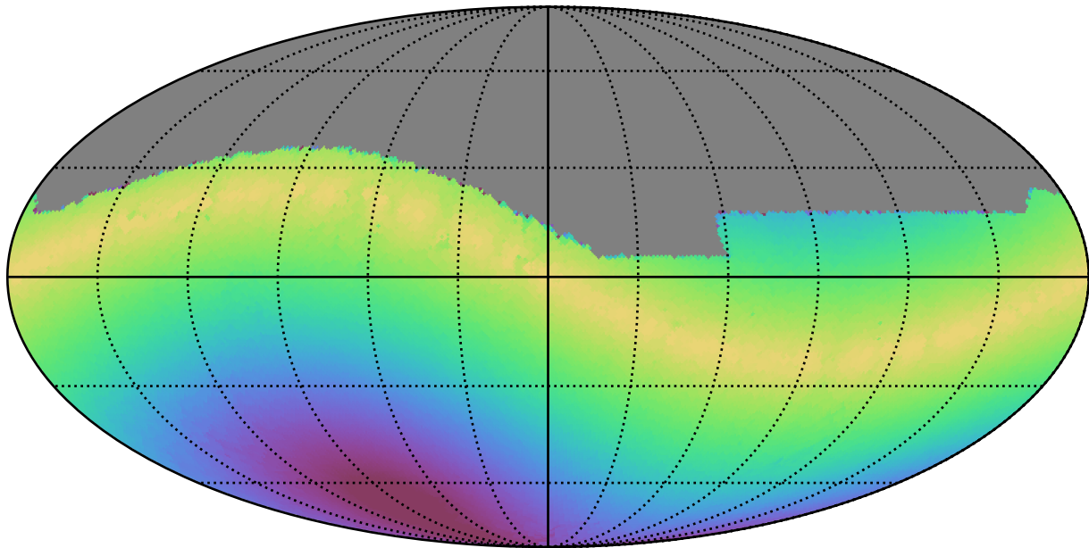
too_100_4v3.4_10yrs All sky g band: Max solarElong
