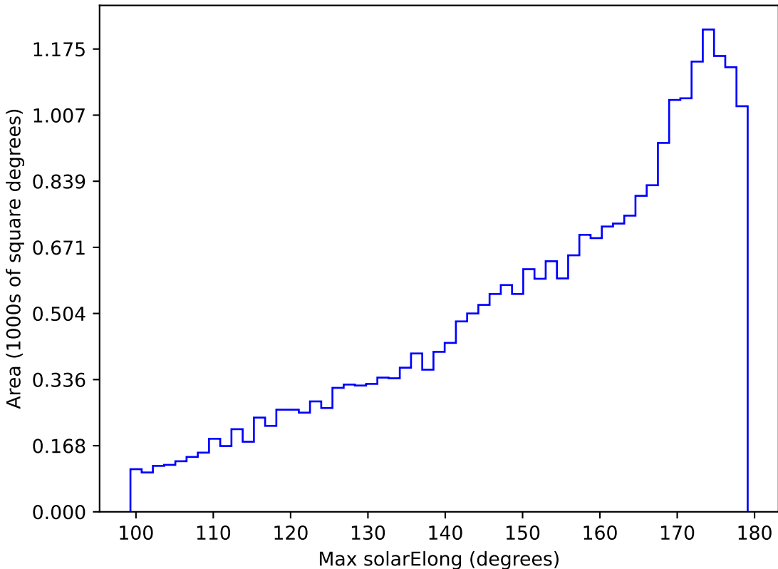
too_100_4v3.4_10yrs All sky g band: Max solarElong
