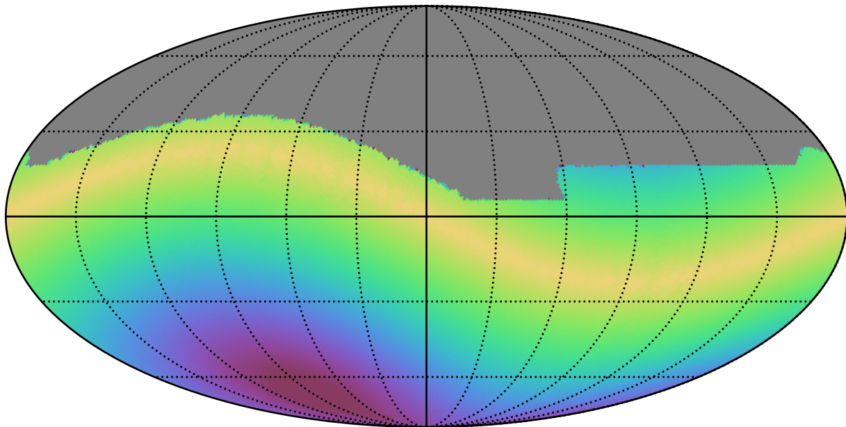
too_100_4v3.4_10yrs All sky all bands: Max solarElong
