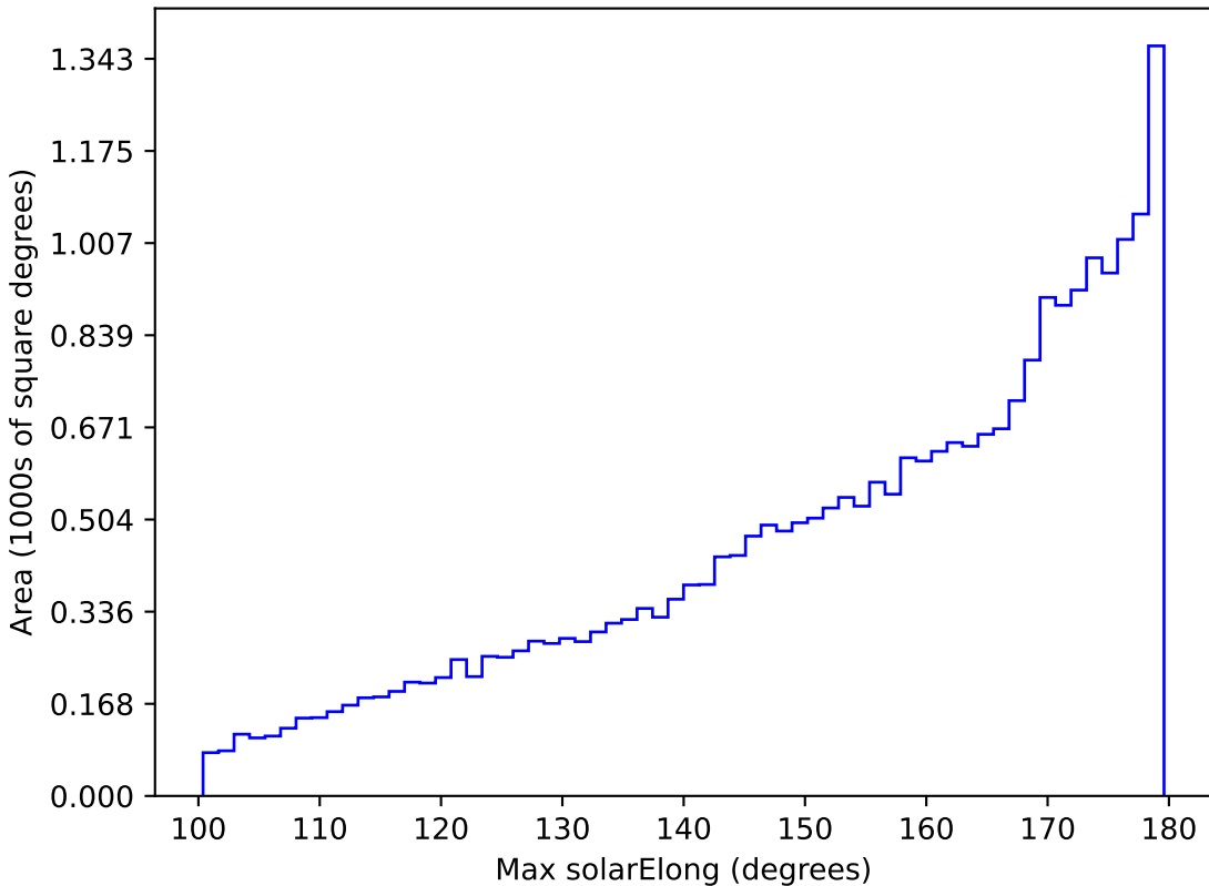
too_100_4v3.4_10yrs All sky all bands: Max solarElong
