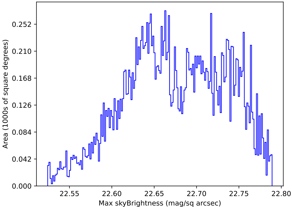
too_100_4v3.4_10yrs Yr 1 u band: Max skyBrightness
