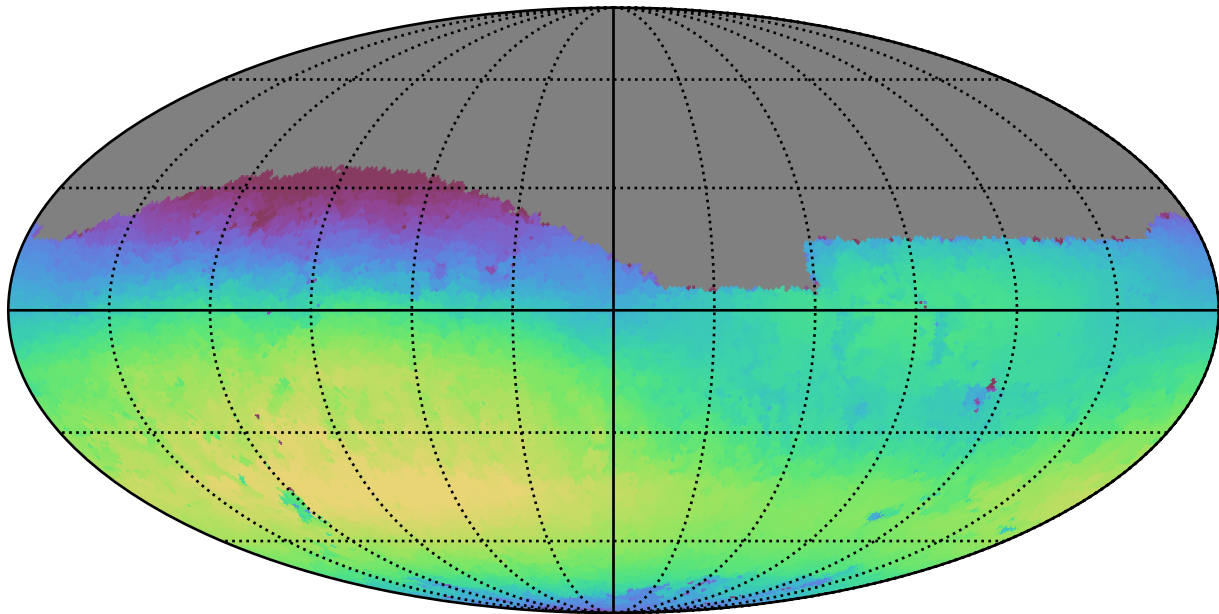
too_100_4v3.4_10yrs Yr 1 r band: Max skyBrightness
