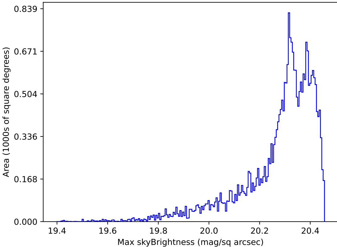
too_100_4v3.4_10yrs Yr 1 i band: Max skyBrightness
