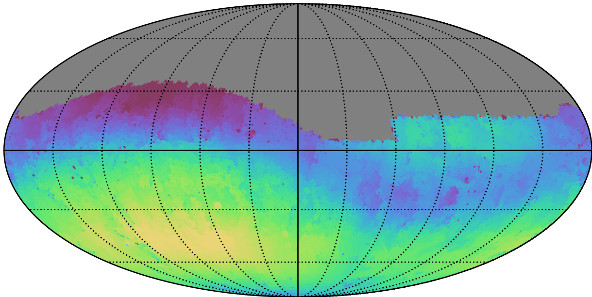
too_100_4v3.4_10yrs Yr 1 g band: Max skyBrightness
