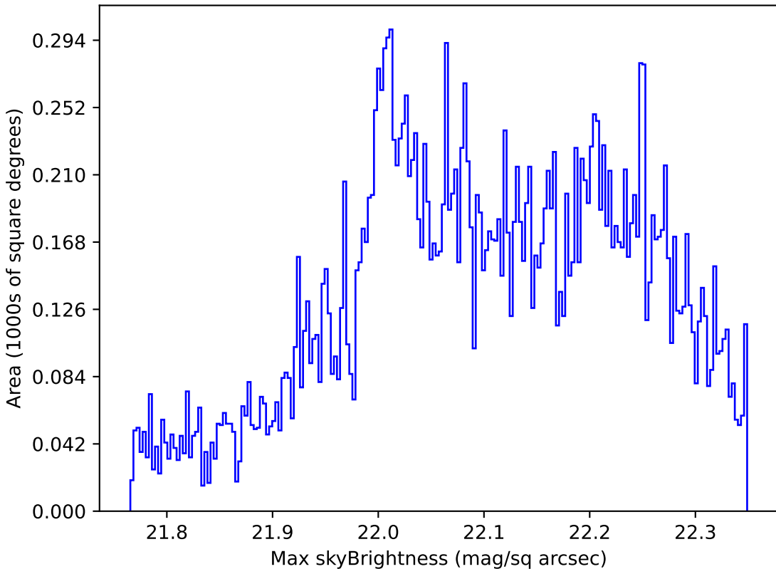
too_100_4v3.4_10yrs Yr 1 g band: Max skyBrightness
