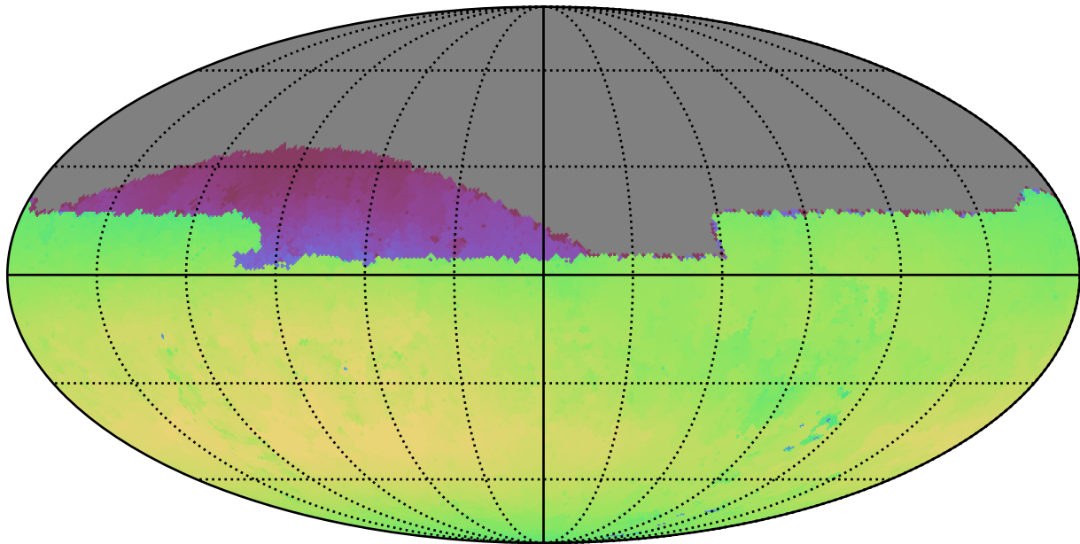
too_100_4v3.4_10yrs Yr 1 all bands: Max skyBrightness
