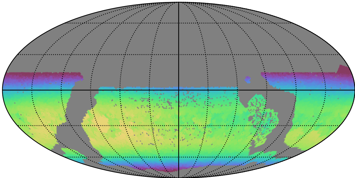
too_100_4v3.4_10yrs WFD z band: Max skyBrightness
