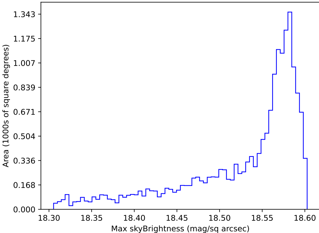
too_100_4v3.4_10yrs WFD y band: Max skyBrightness
