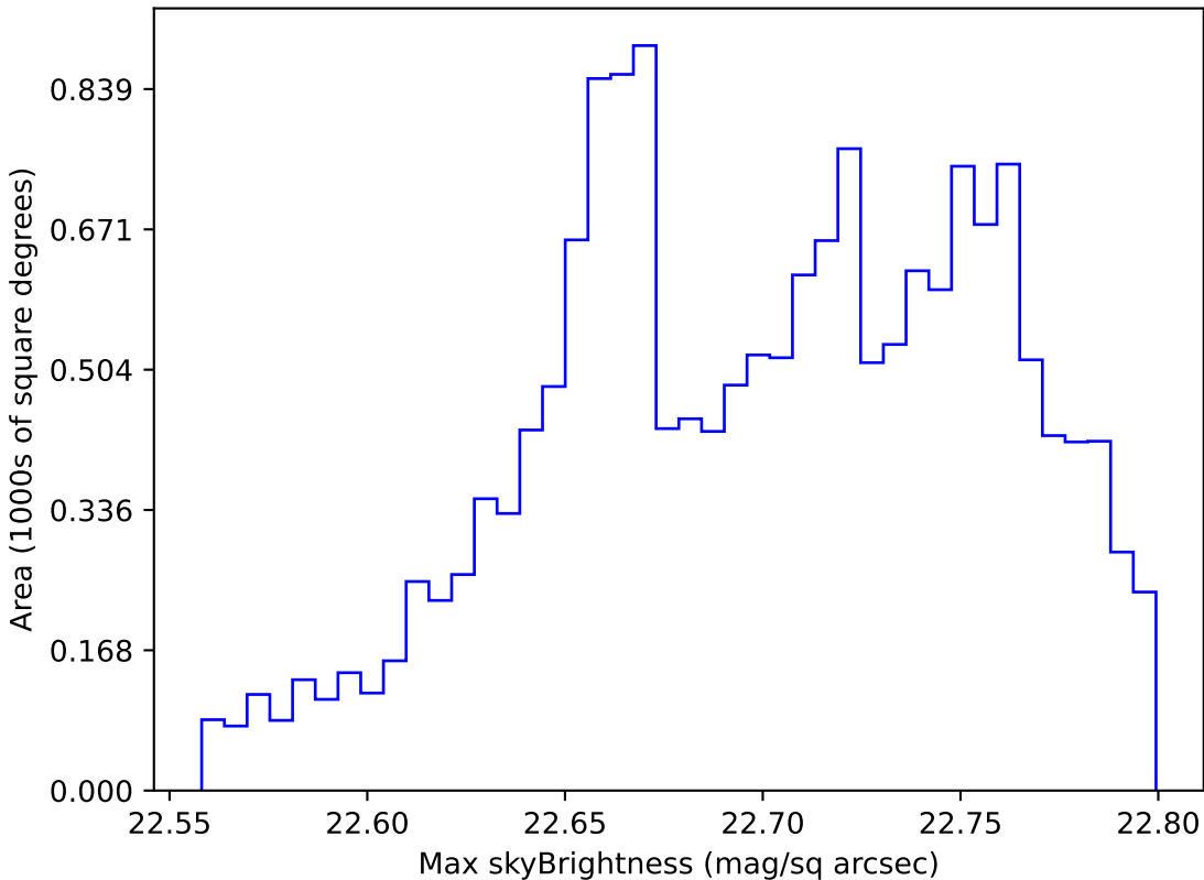
too_100_4v3.4_10yrs WFD u band: Max skyBrightness
