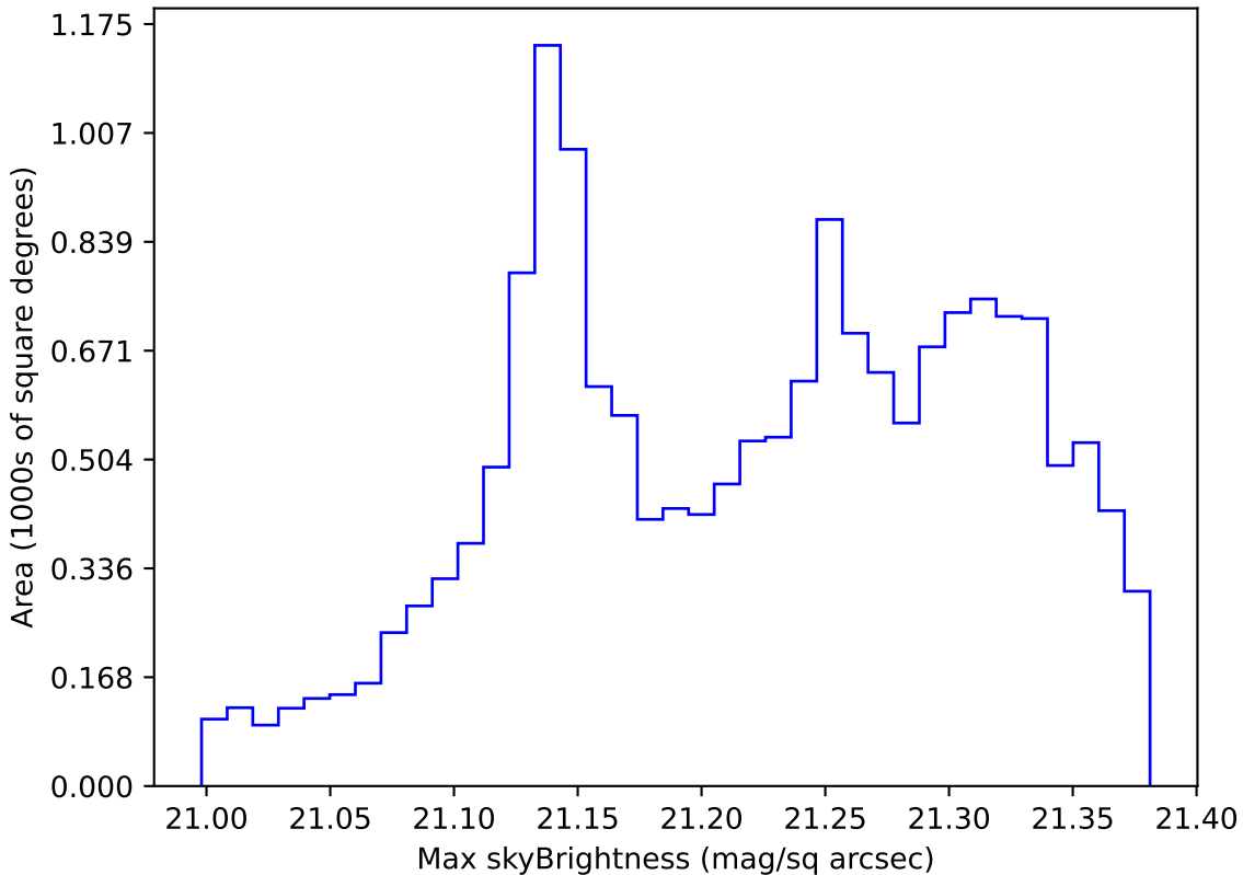
too_100_4v3.4_10yrs WFD r band: Max skyBrightness
